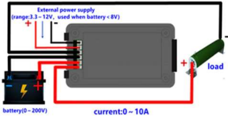
Figure 12 PZEM-013 Wiring Diagram
