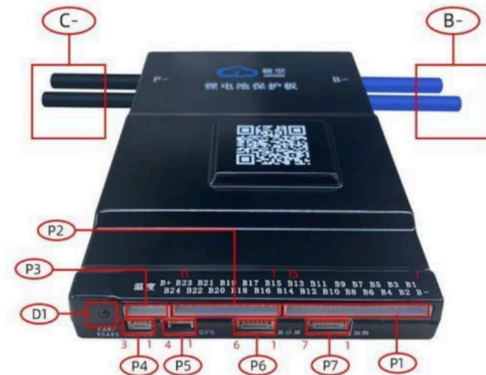
Obr. 1 Schéma konektoru BD6AxxS-10P/ B1AxxS-15P/B2AxxS-15P/B2AxxS20P
