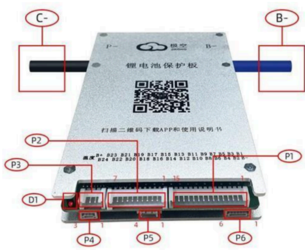
Obr. 2 Schéma konektoru BD6AxxS-6P/ BD6AxxS8P
