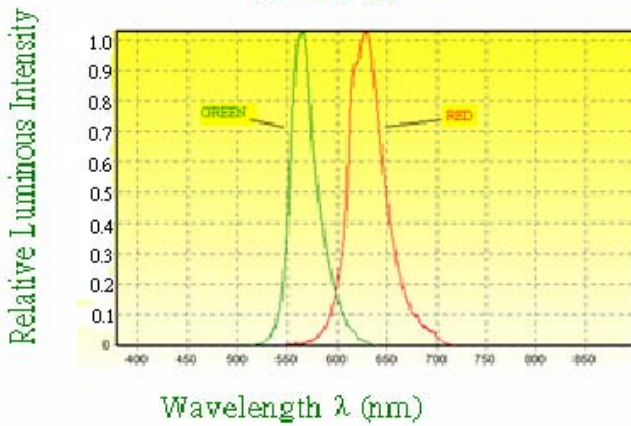
Wavelength Characteristics (Ta=25°C)
