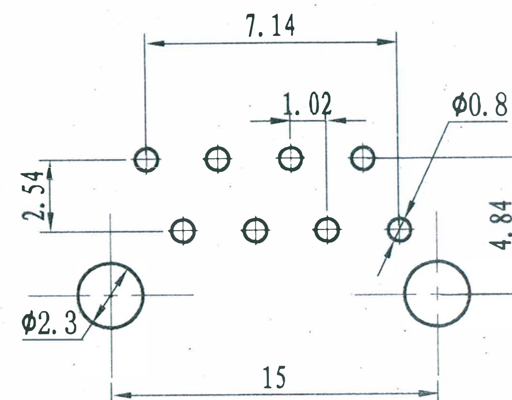
PC board hole positions
